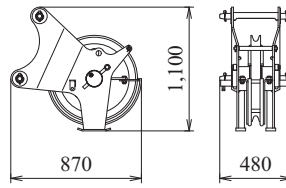
Auxiliary Sheave Weight: 195 kg
