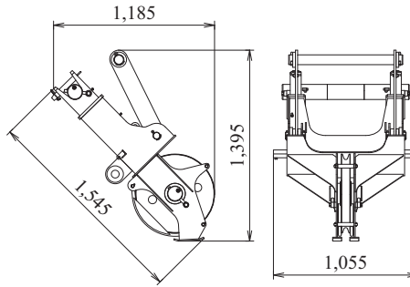
2 Part-line Aux. Sheave (Optional) Weight: 470 kg
